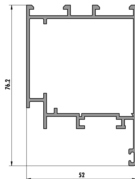
6214 (1,088 kg/m)
