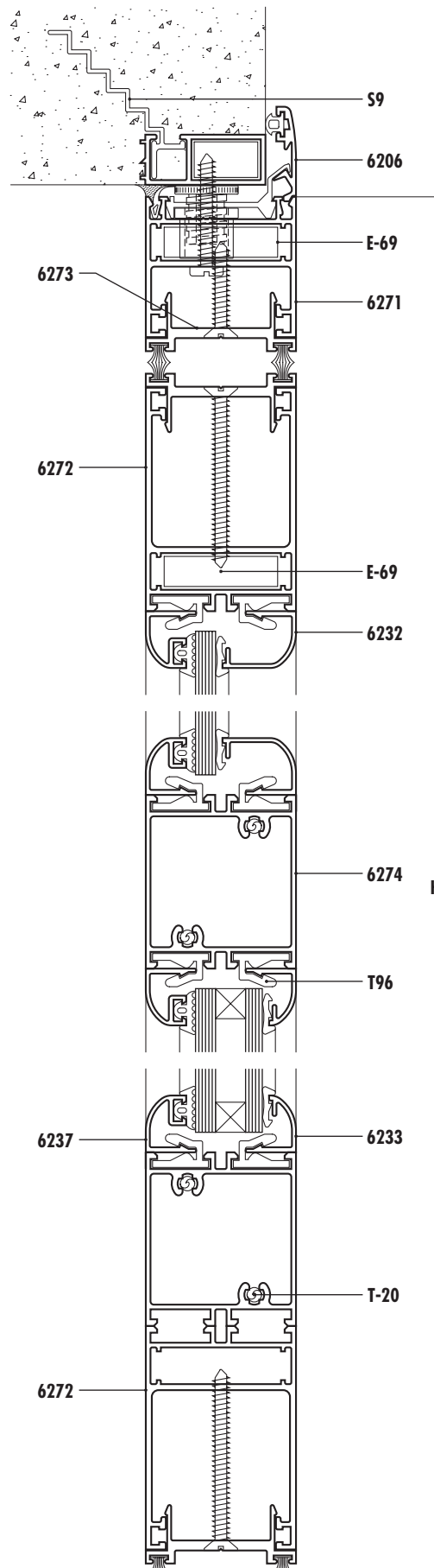
PVVC Corte 6-7-8
