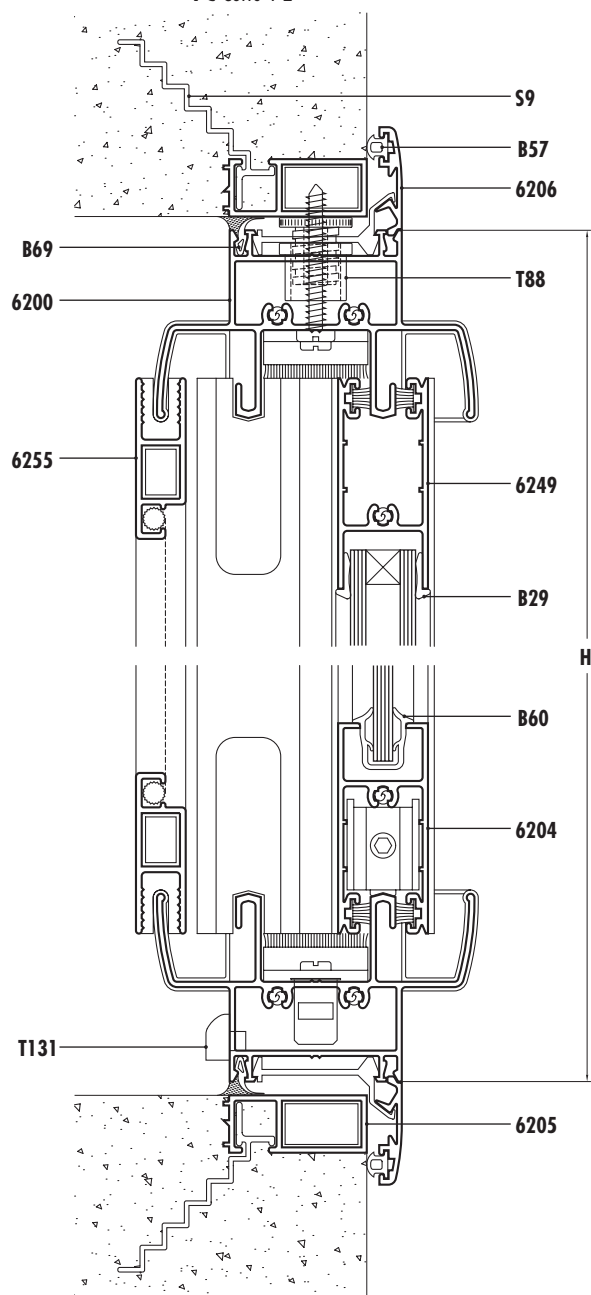
VC Corte 1-2
