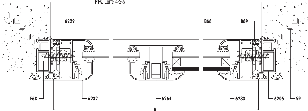
PFC Corte 4-5-6
