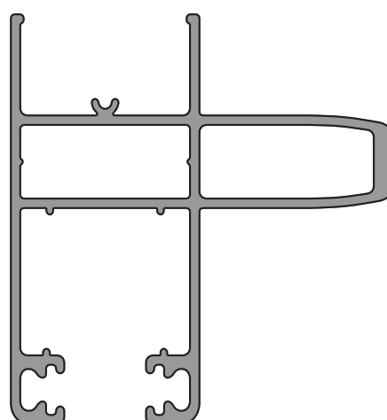
6911 (1,126 Kg/m)
