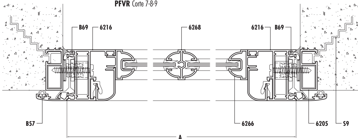
PFVR Corte 7-8-9
