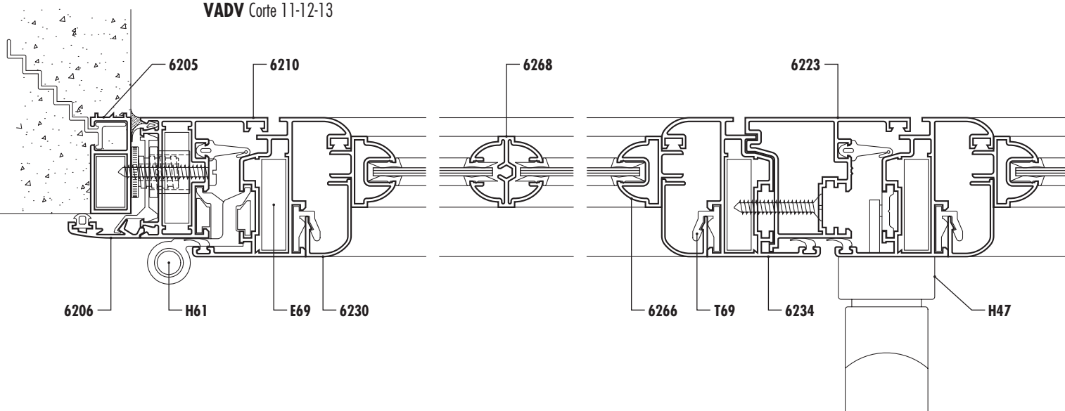
VADV Corte 11-12-13
