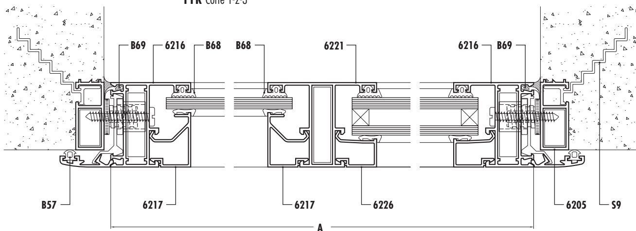
PFR Corte 1-2-3
