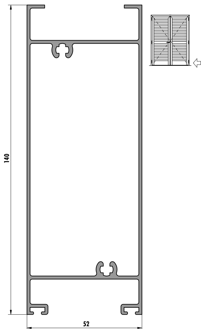
6281 (1,760 kg/m)
