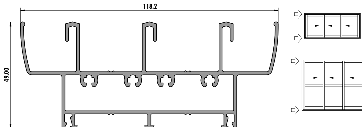
6240 (1,841 kg/m)
