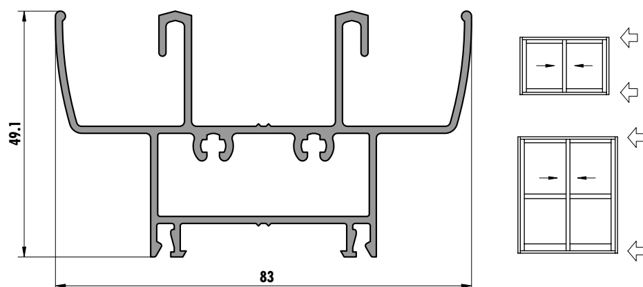
6200 (1,266 kg/m)
