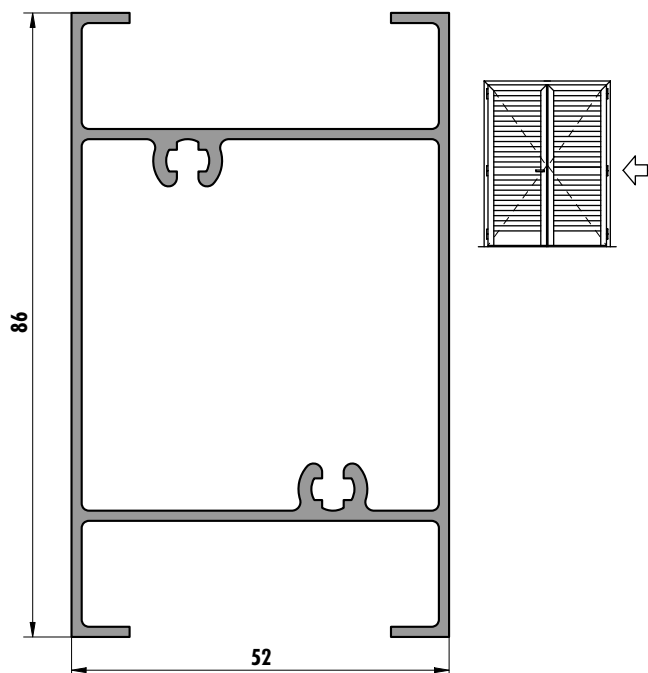
6276 (1,301 kg/m)
