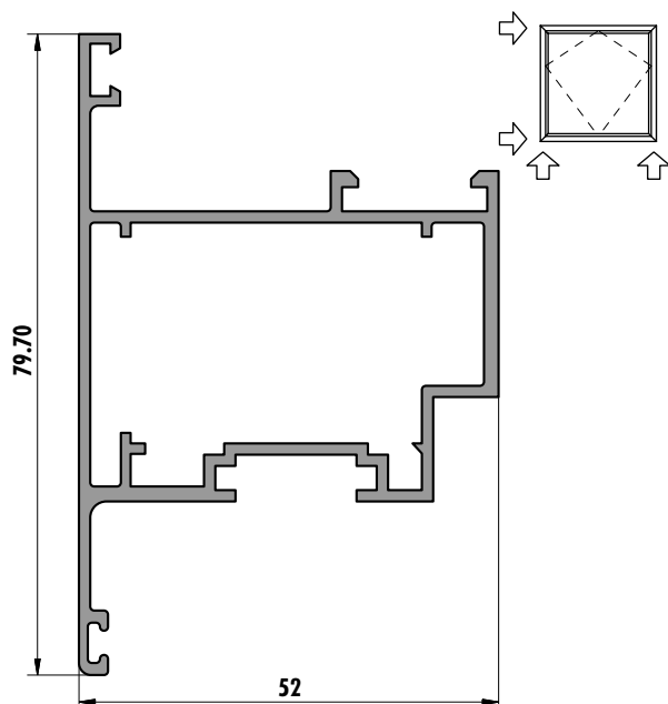
6258 (1,061 kg/m)
