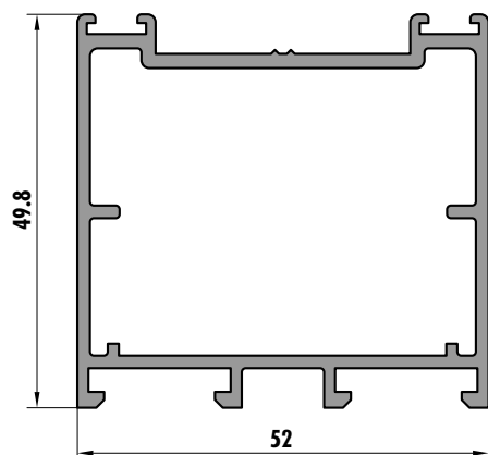
6285 (1,040 kg/m)
