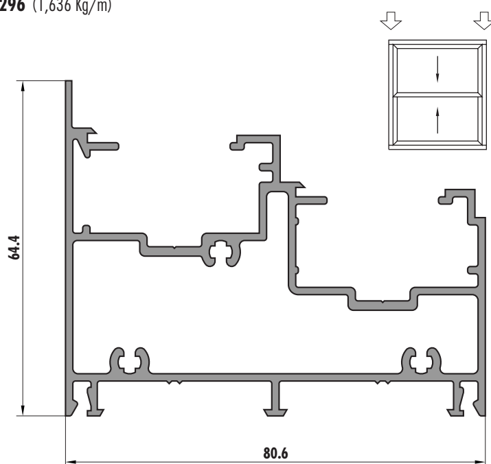
6296 (1,636 Kg/m)
