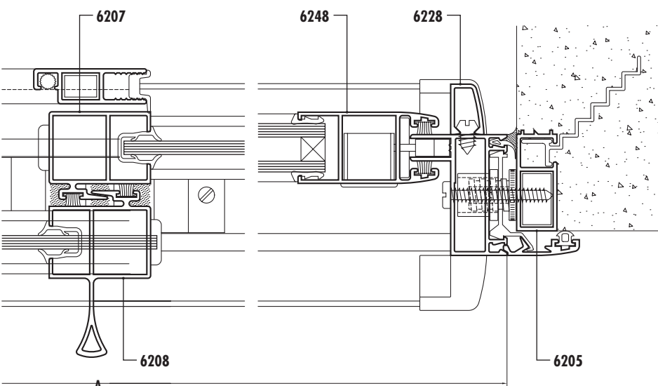
VC Corte 1-2
