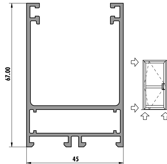
6272 (1,156 kg/m)
