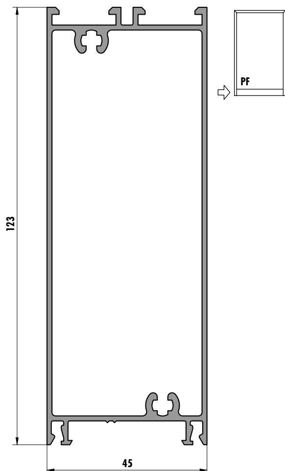
6263 (1,679 kg/m)
